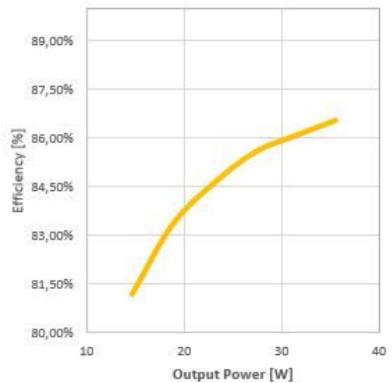
Typical Efficiency vs Load (230 V / 50 Hz)
